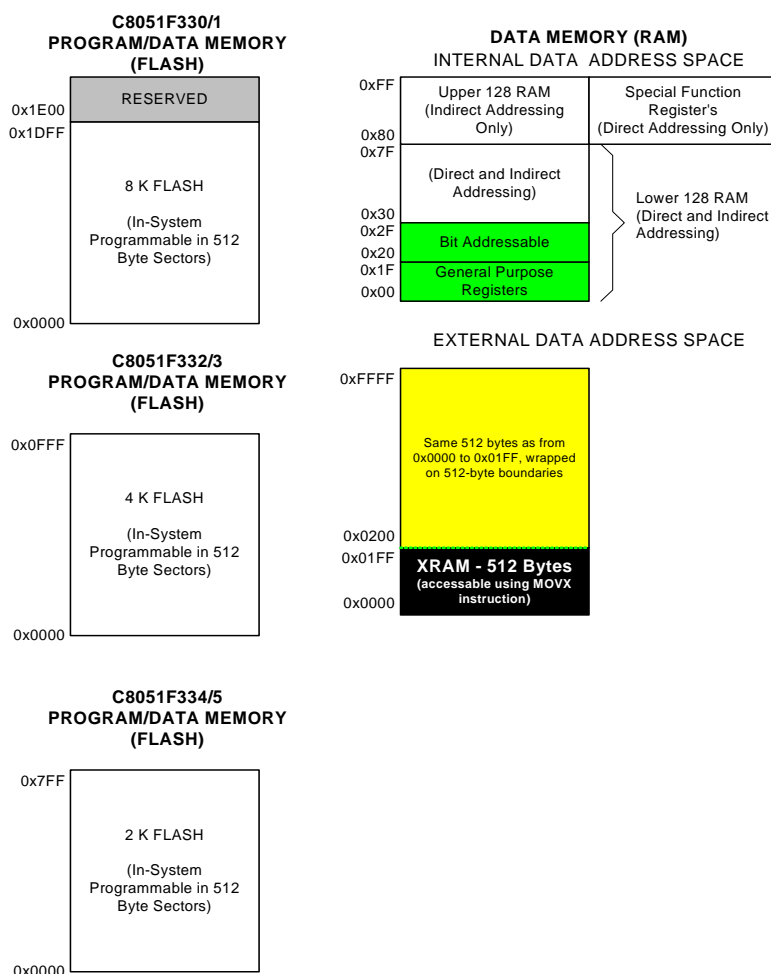
Figure 9.2. Memory Map
